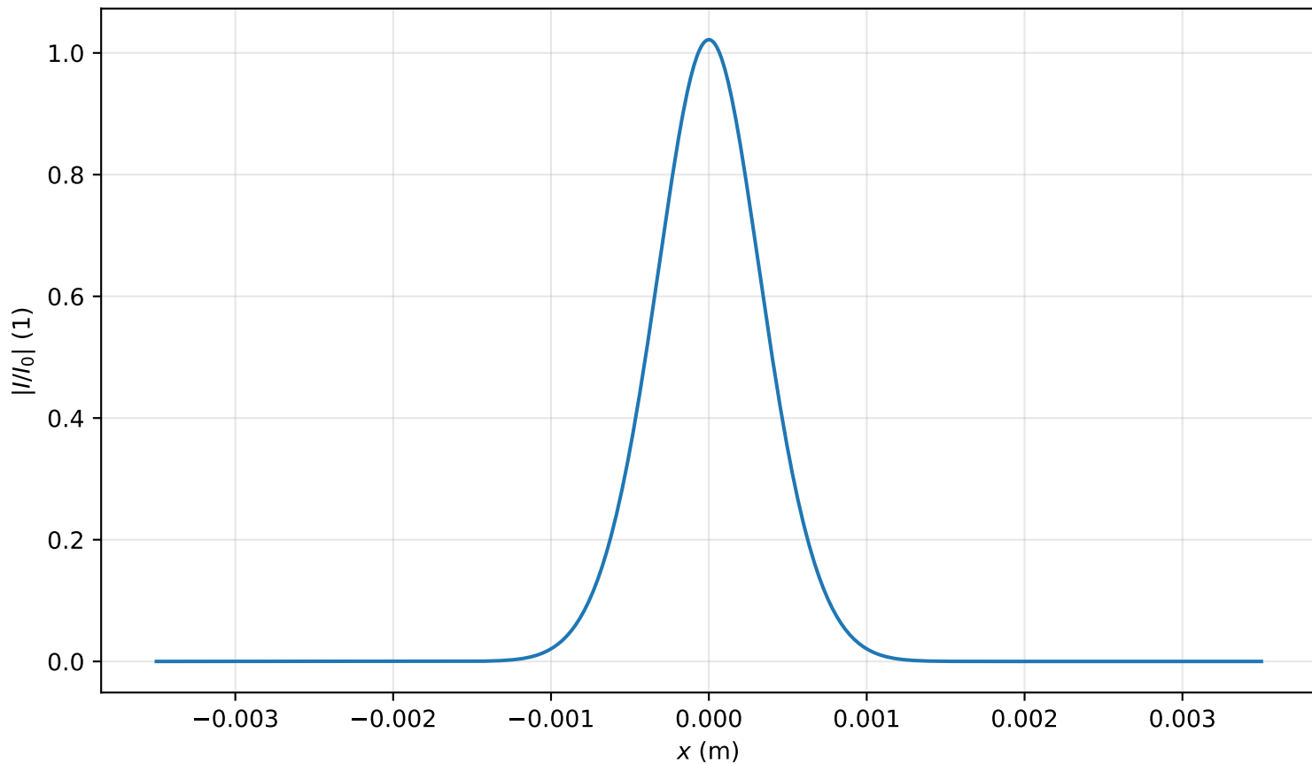
Intensity profile I(x, y = 0, z = 0.557m)/I_0 , P_{in}=0.4P_{cr} , artificial time
